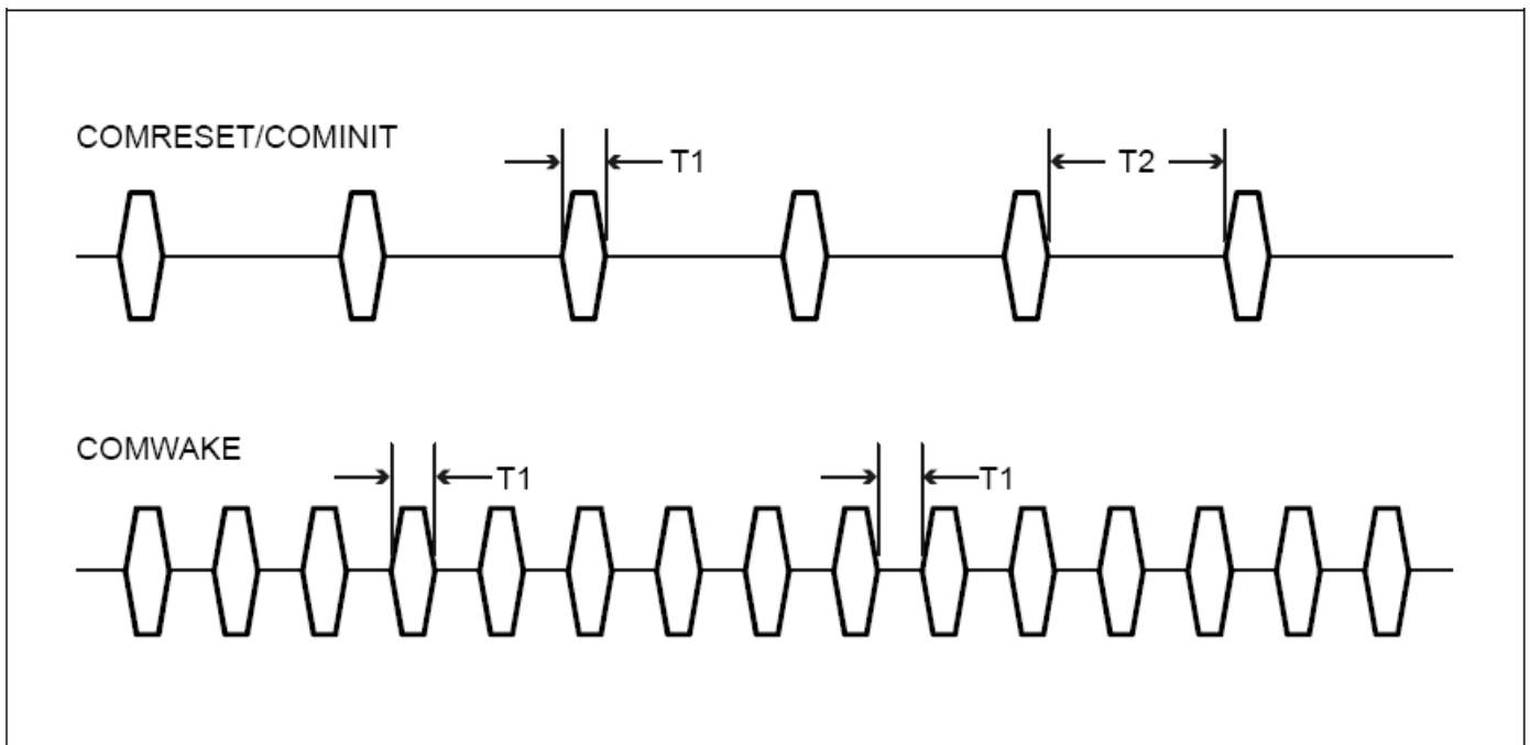
Figure 4: OOB signals
