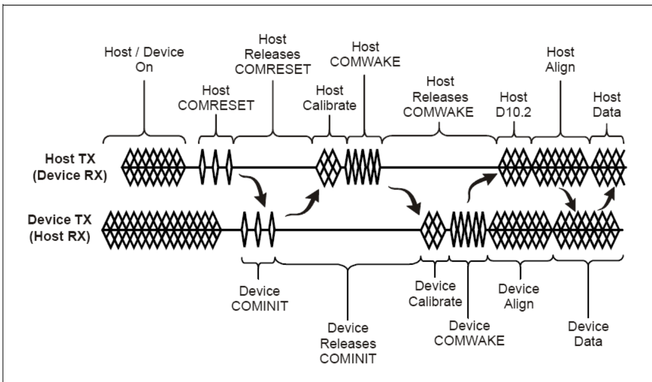
Figure 5 : comreset sequence
