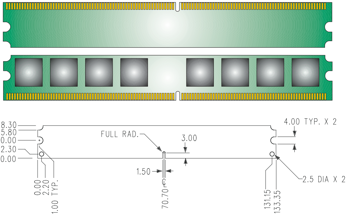
Figure 1: KVR800D2N6/1G 240-Pin DIMM
